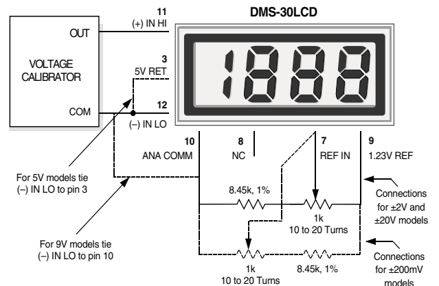
Figure 9. External Gain Adjustment
