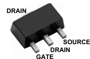
TO-243AA (SOT-89)
