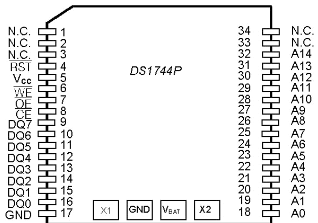
PowerCap Module BOARD (Uses DS9034PCX PowerCap)
