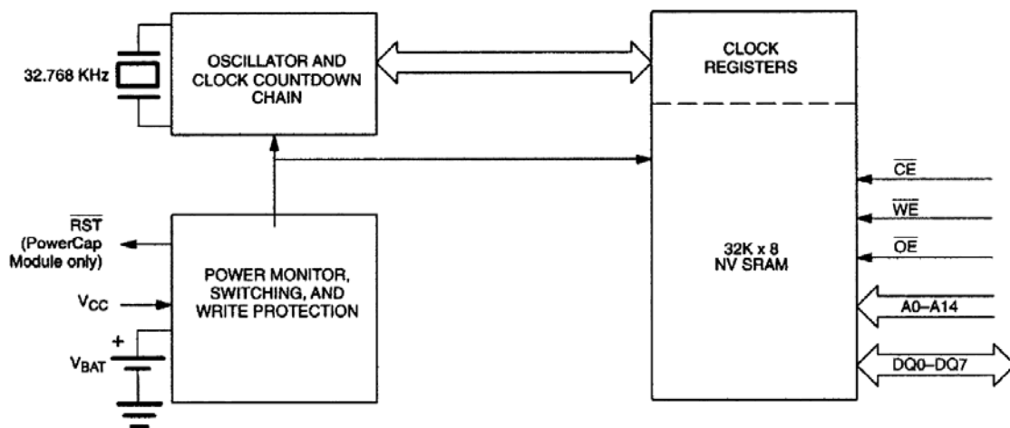
Figure 1. Block Diagram
