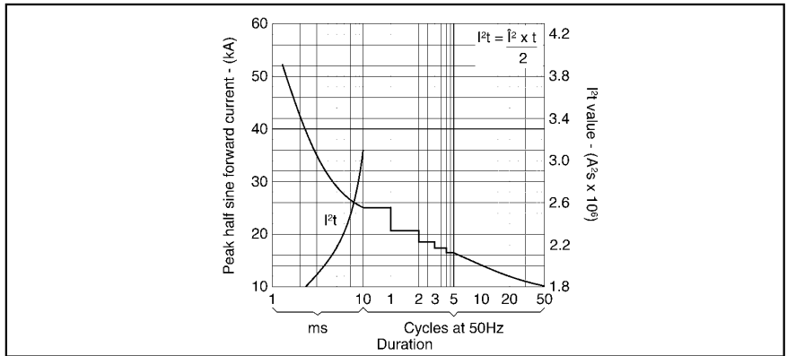
Surge (non-repetitive) forward current vs time ( T_{case} = 175^\circ\text{C} )
