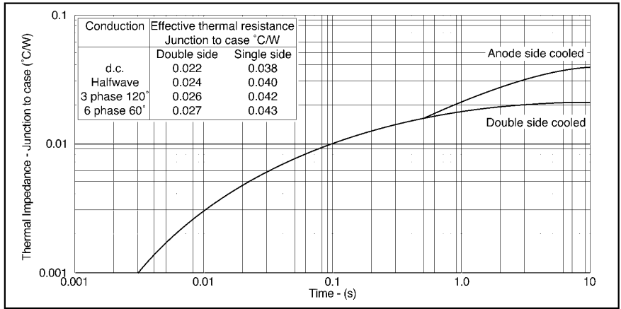
Maximum (limit) transient thermal impedance - junction to case - (°C/W)
