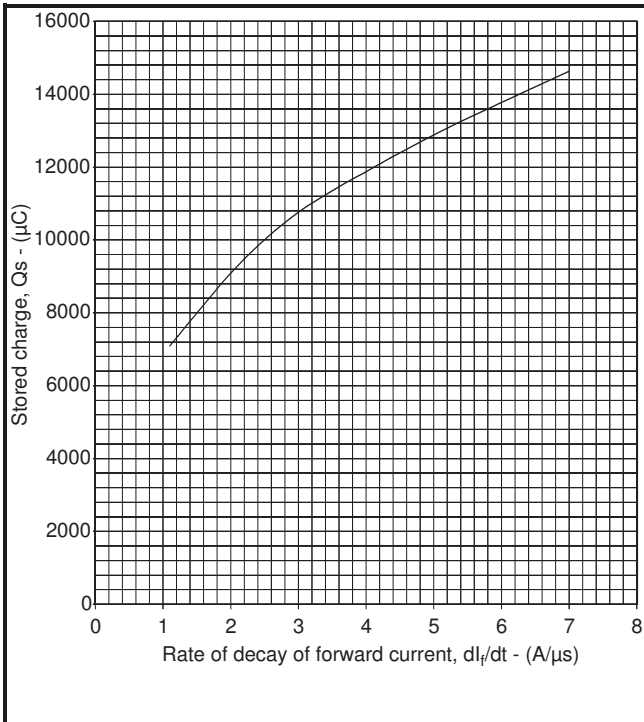
Fig.4 Stored charge
