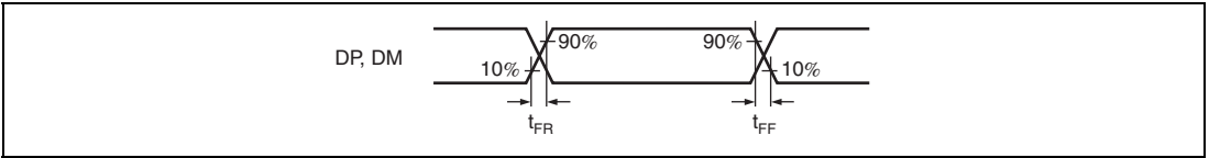
Figure 31.74 DP and DM Output Timing (Full-Speed)
