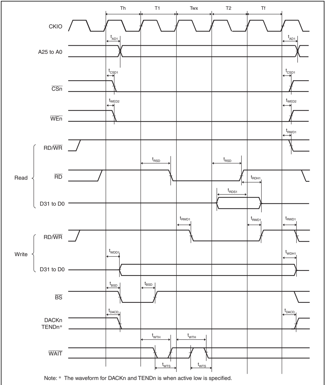
Figure 31.20 Bus Cycle of SRAM with Byte Selection (SW = 1 Cycle, HW = 1 Cycle, One Asynchronous External Wait Cycle, BAS = 1 (Write Cycle WE Control))
