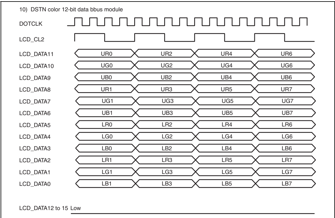
Figure 24.19 Clock and LCD Data Signal Example (DSTN Color 12-Bit Data Bus Module)
