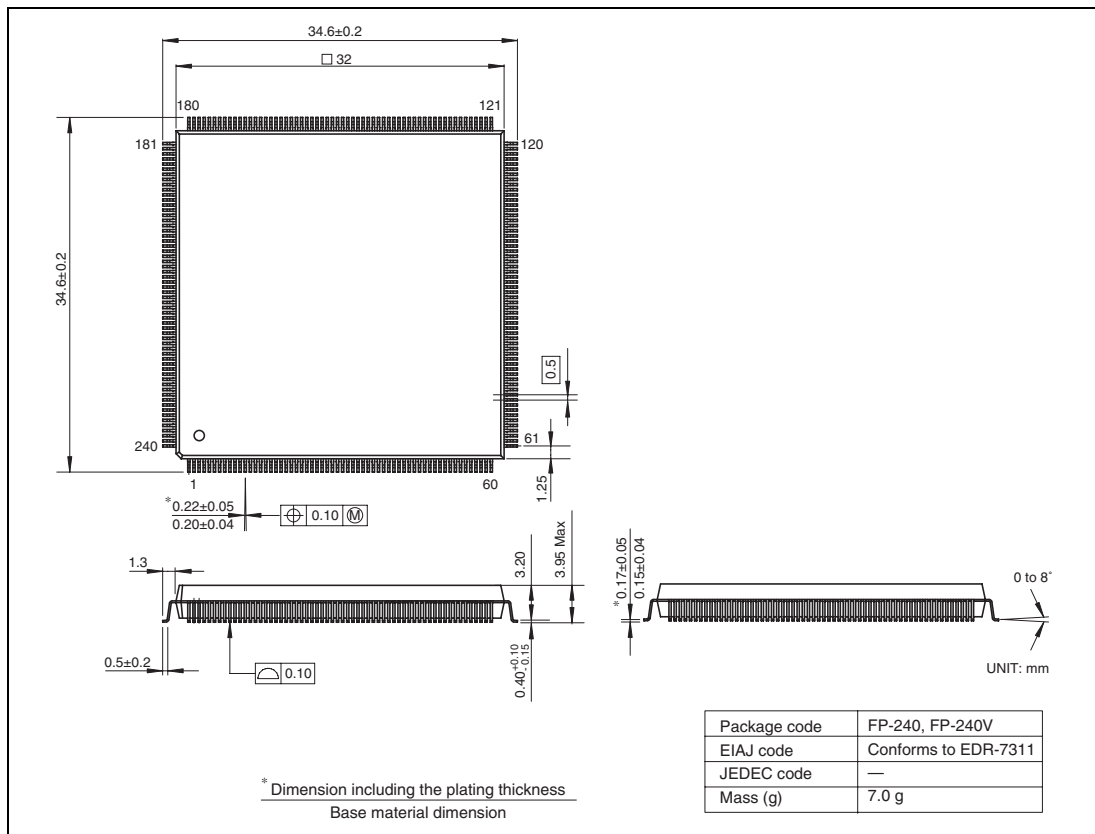
Figure C.1 Package Dimensions
