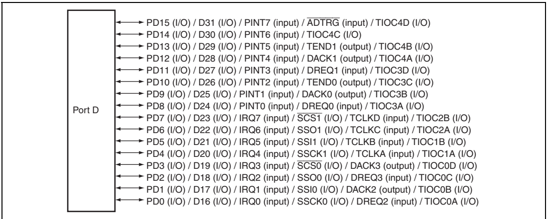
Figure 26.4 Port D
