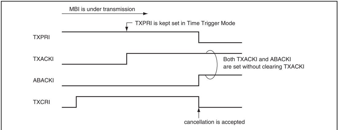
Figure 19.7 TXACK and ABACK in Time Trigger Transmission
