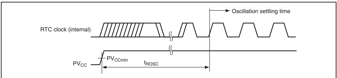
Figure 31.8 RTC Clock Oscillation Settling Time
