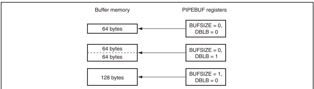
Figure 23.10 Example of Buffer Memory Settings
