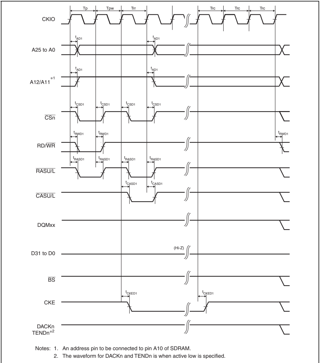
Figure 31.37 Synchronous DRAM Self-Refreshing Timing (WTRP = 1 Cycle)
