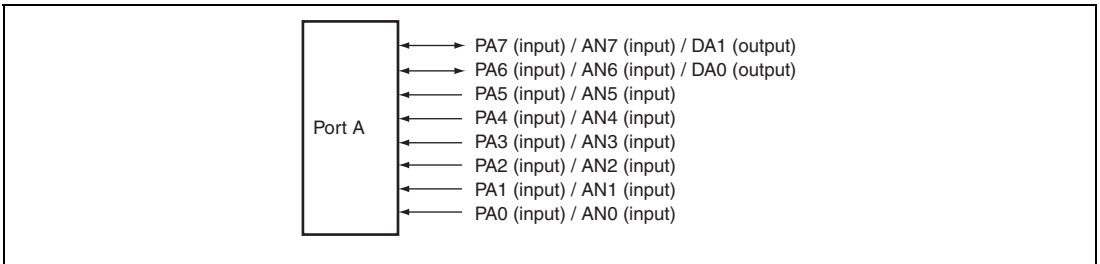
Figure 26.1 Port A
