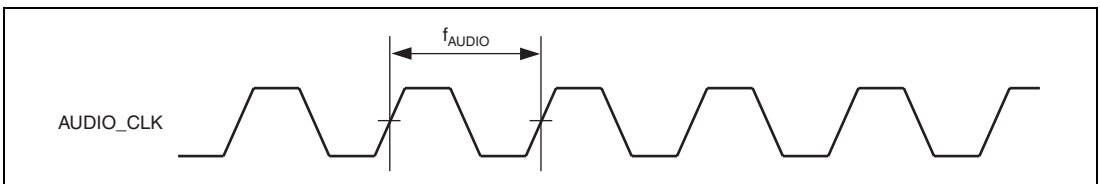
Figure 31.61 AUDIO_CLK Input Timing
