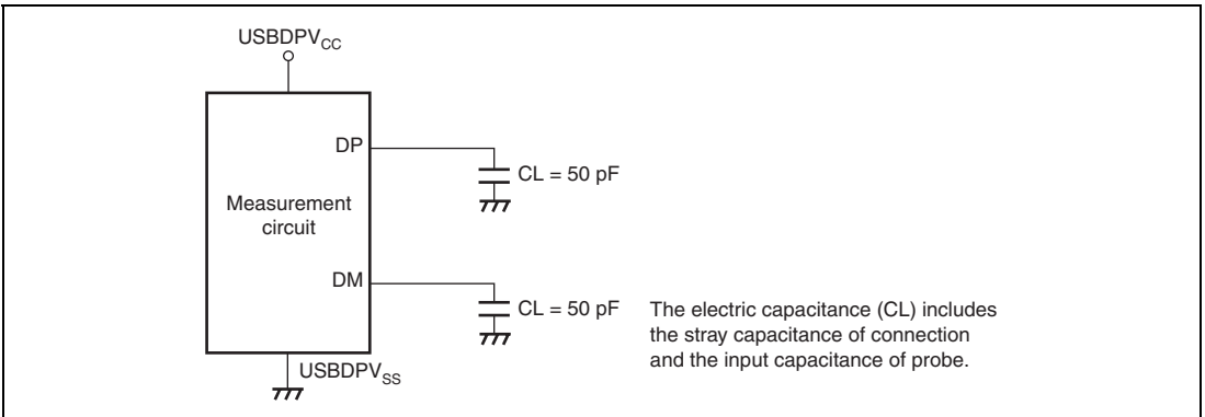
Figure 31.75 Measurement Circuit (Full-Speed)
