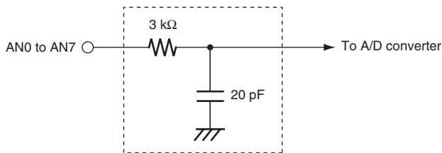
Figure 20.9 Analog Input Pin Equivalent Circuit
