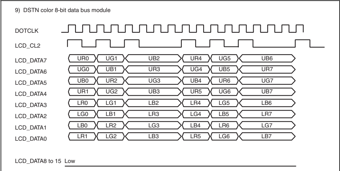
Figure 24.18 Clock and LCD Data Signal Example (DSTN Color 8-Bit Data Bus Module)
