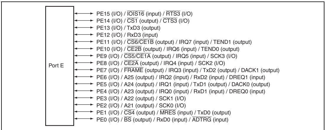
Figure 26.5 Port E
