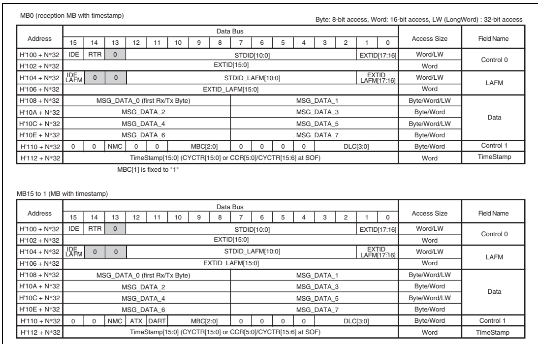
Figure 19.3 Mailbox-N Structure
