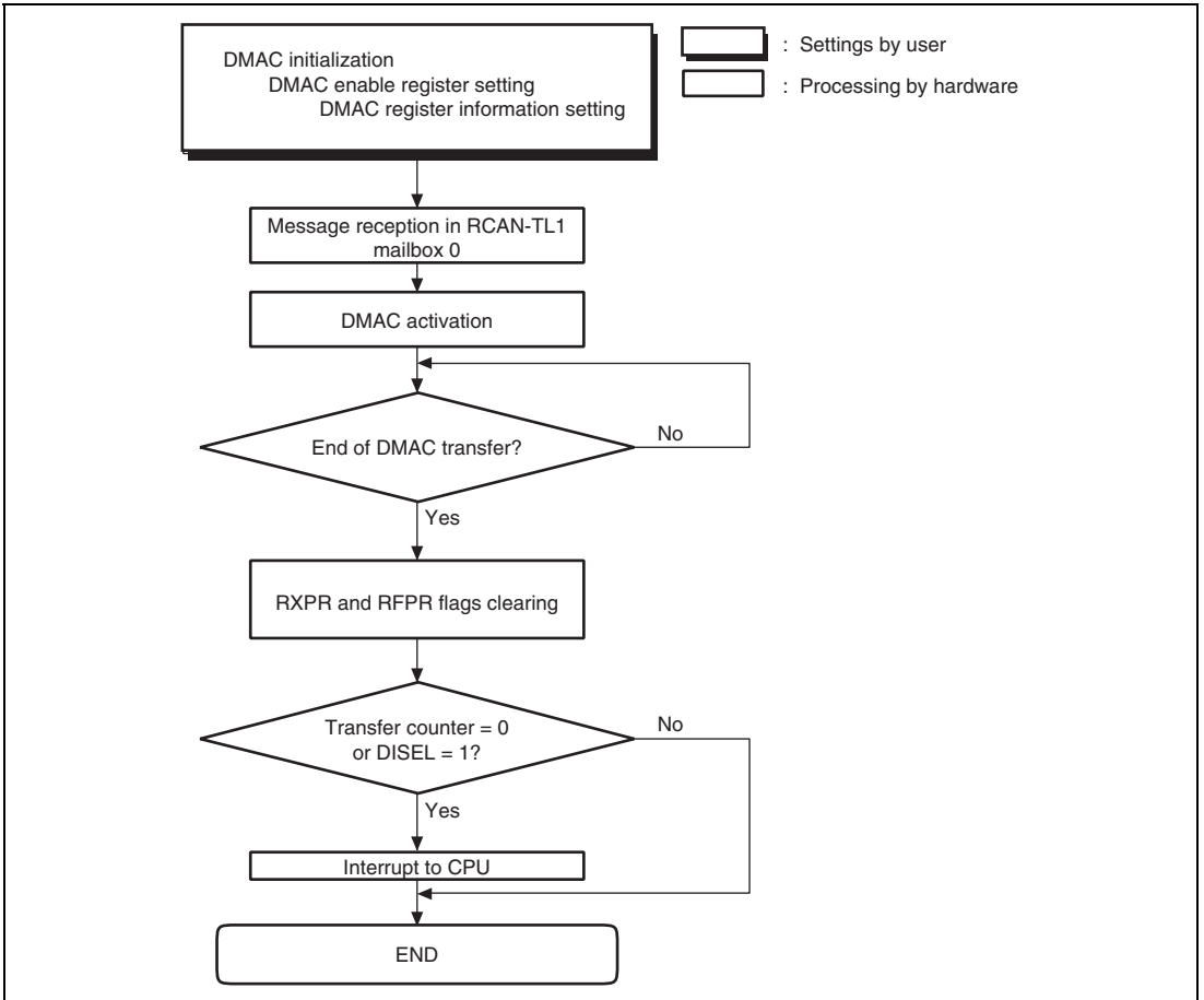
Figure 19.26 DMAC Transfer Flowchart
