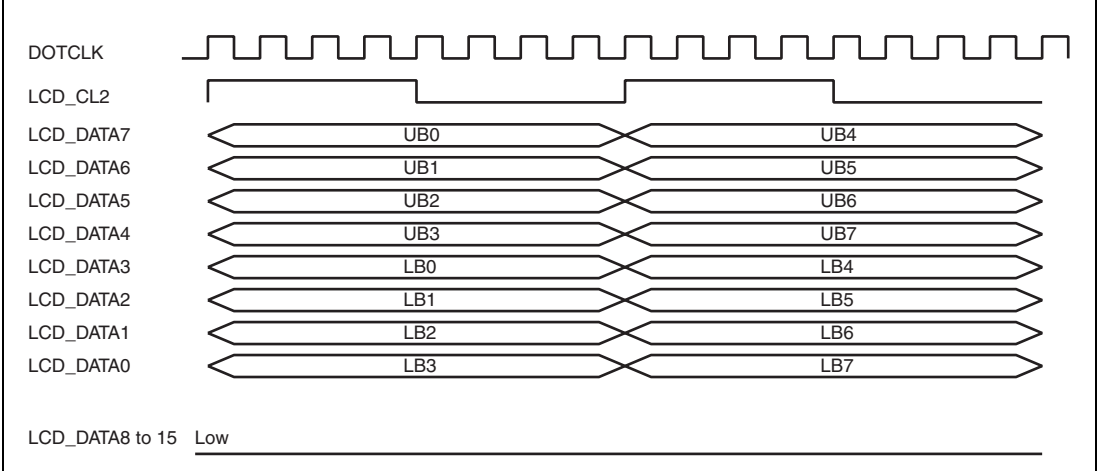
Figure 24.16 Clock and LCD Data Signal Example (DSTN Monochrome 8-Bit Data Bus Module)
