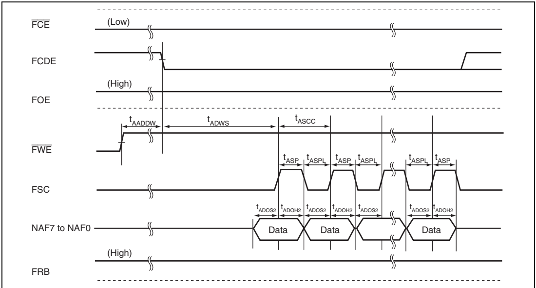
Figure 31.67 AND Type Flash Memory Data Write Timing
