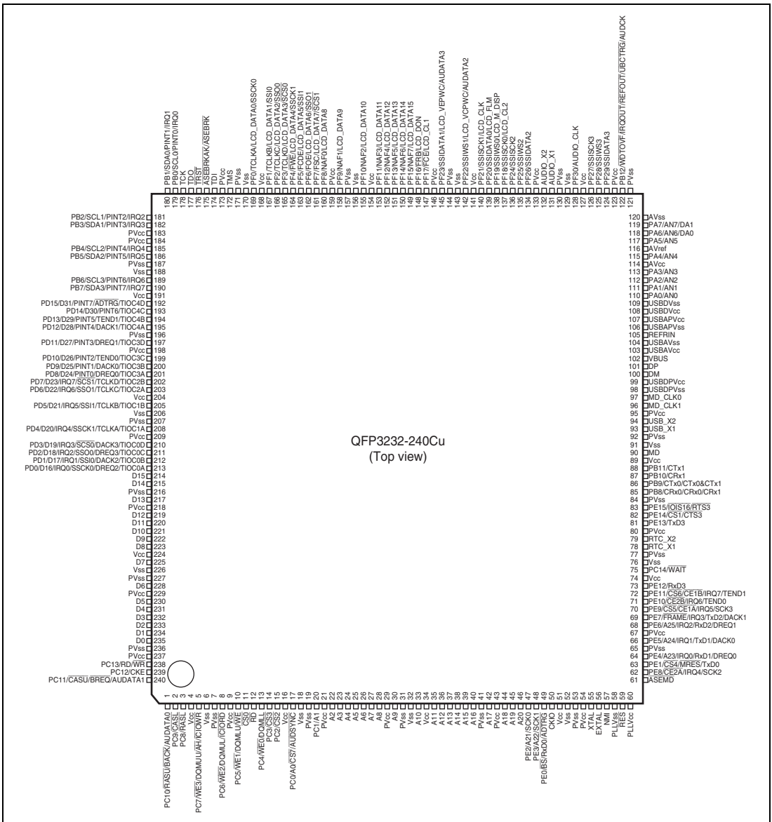
Figure 1.2 Pin Arrangement
