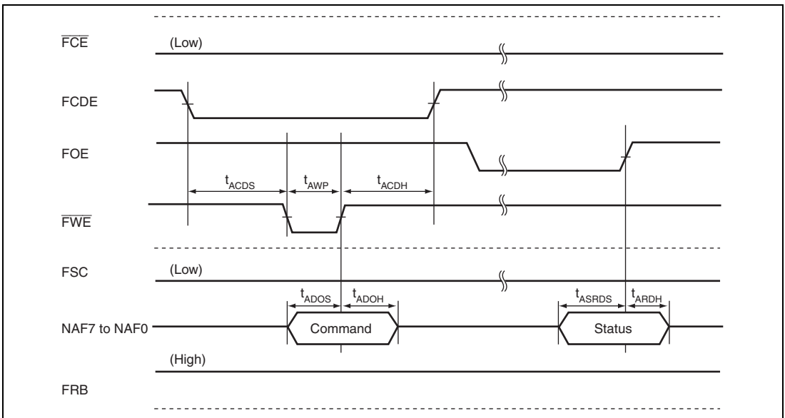
Figure 31.68 AND Type Flash Memory Status Read Timing
