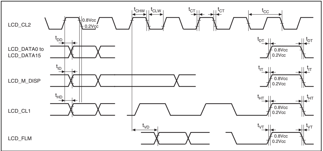
Figure 31.78 LCDC Module Timing
