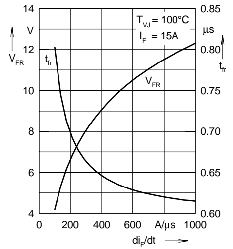
Fig. 6 Peak forward voltage V_{FR} and t_{rr}
