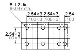
PC board pattern (Copper-side view) Single side stable
