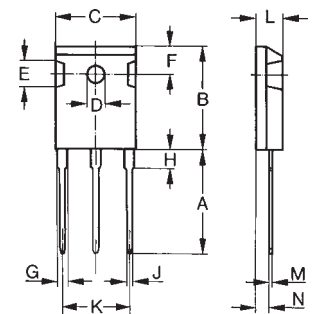
TO-247 AD and ISOPLUS 247™
