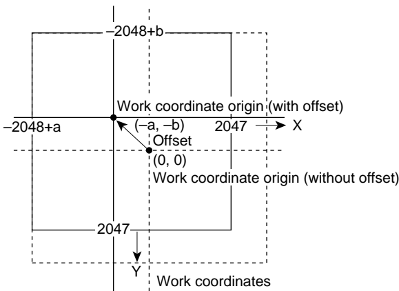
Figure 3.20 Work Coordinates
