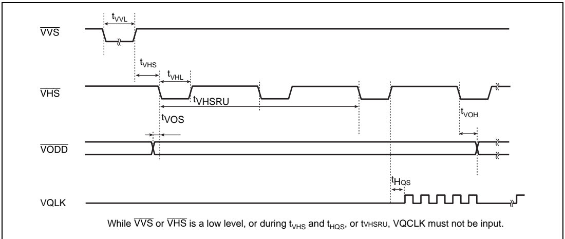
Figure 7.14 (2) Video Interface Timing
