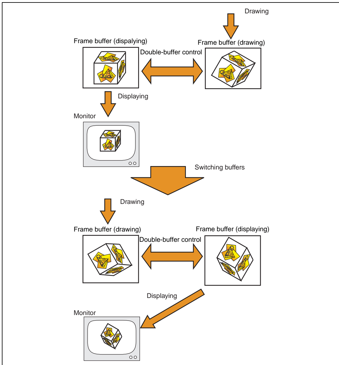
Figure 1.4 Double-Buffering Architecture
