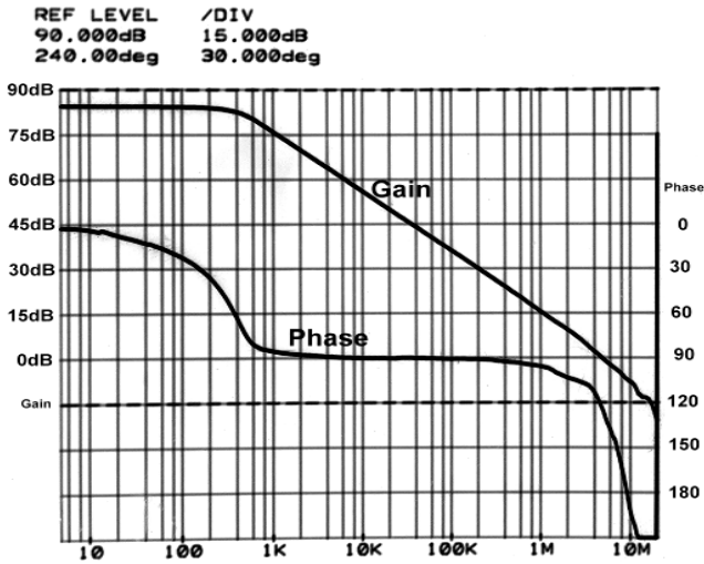
Figure (f) Open Loop Gain & Phase vs. Frequency
