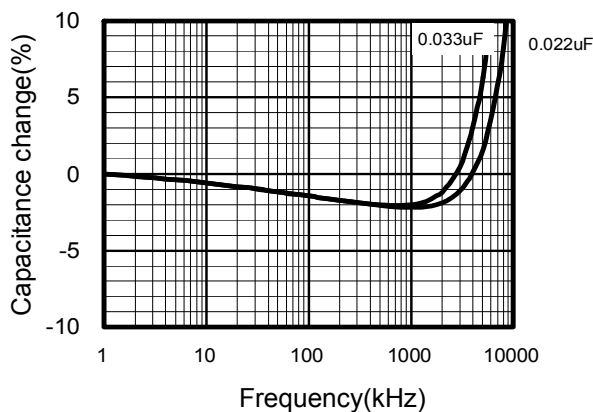
Frequency Characteristics
