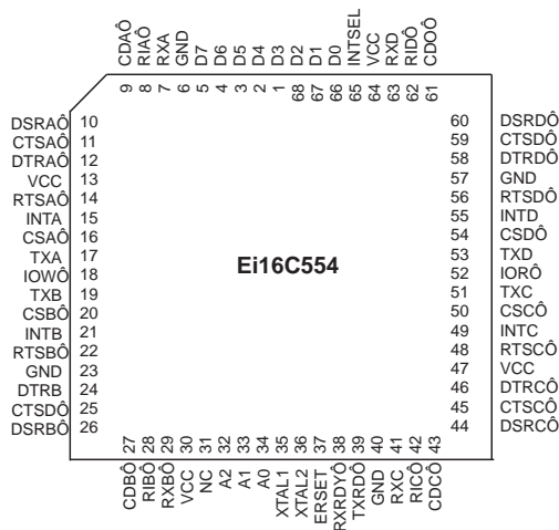
68-PIN PLCC
