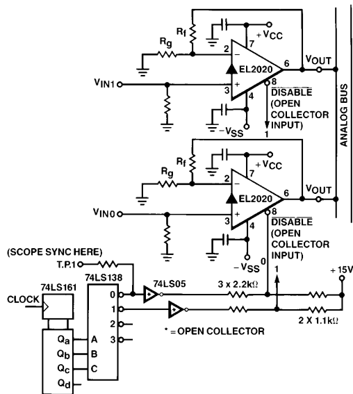
Using the EL2020 as a Multiplexer
