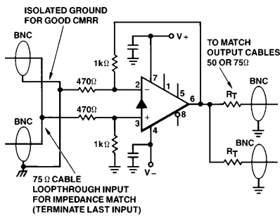
Video Distribution Amplifier with Difference Input
