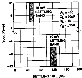
Settling Time
