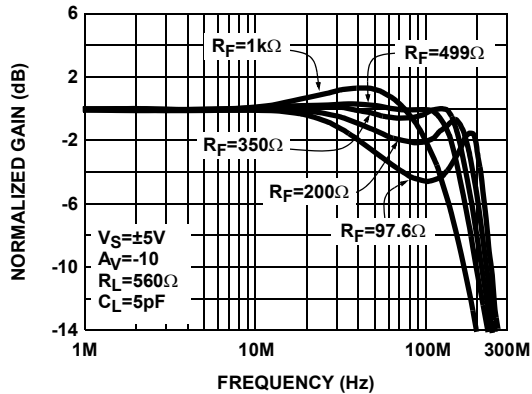
FIGURE 3. INVERTING FREQUENCY RESPONSE FOR VARIOUS R_F
