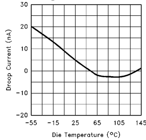
Drop Current vs Temperature (Sample & Hold)
