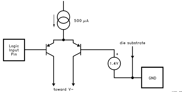
Figure 1. Simplified Logic Input Circuitry
