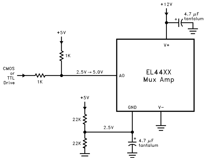
Figure 2. Using the EL44XX Mux Amps with +5\text{V} and +12\text{V} Supplies
