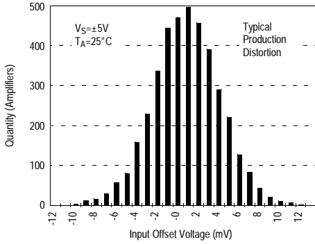
EL5410C Input Offset Voltage Distribution
