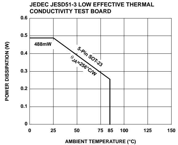
FIGURE 11. PACKAGE POWER DISSIPATION vs AMBIENT TEMPERATURE
