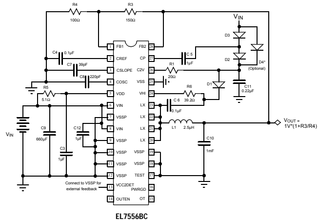
EL7556BC C12 - 1µF C3, C4, C5, C6, C7 C8 - ceramic C5, C11 - ceramic or tantalum C9 - Sprague 293D337X96R3 2X330µF C10 - Sprague 293D337X96R3 3X330µF L1 - Pulse Engineering, PE-53661 D1-D4: BAT54S fast diode D4 Required for EL7556ACM Only
