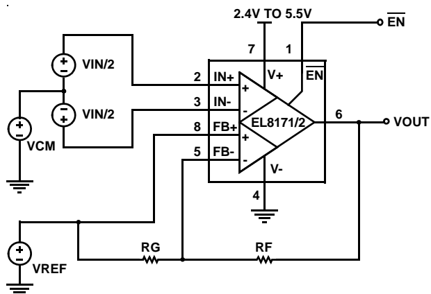
FIGURE 41. CIRCUIT 3 - REFERENCE CONNECTION WITH AN AVAILABLE VREF
