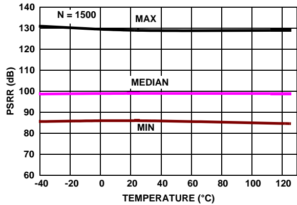
FIGURE 28. EL8172 PSRR vs TEMPERATURE, V_+, V_- = \pm 1.2V \text{ TO } \pm 2.5V
