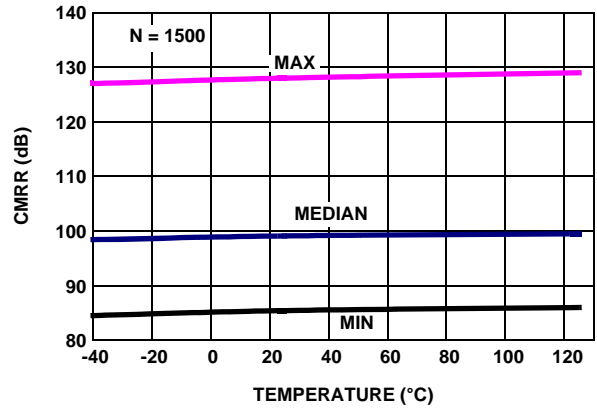
FIGURE 26. EL8172 CMRR vs TEMPERATURE, V_{CM} = +2.5V \text{ TO } -2.5V, V_+, V_- = \pm 2.5V
