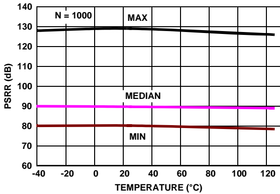
FIGURE 27. EL8171 PSRR vs TEMPERATURE, V_+, V_- = \pm 1.2V \text{ TO } \pm 2.5V
