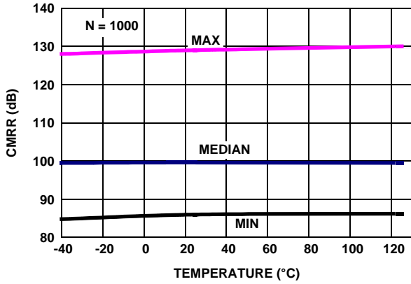
FIGURE 25. EL8171 CMRR vs TEMPERATURE, V_{CM} = +2.5V \text{ TO } -2.5V, V_+, V_- = \pm 2.5V
