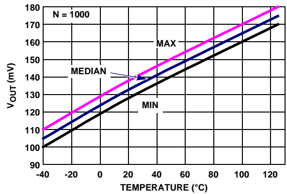
FIGURE 34. EL8172 V_{OUT} LOW vs TEMPERATURE, R_L = 1k, V_+, V_- = \pm 2.5V
