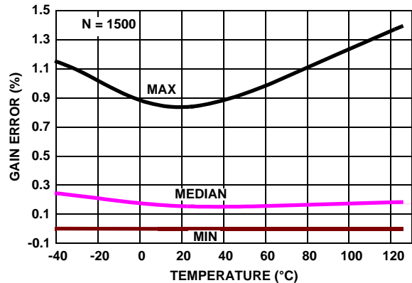
FIGURE 30. EL8172% GAIN ERROR vs TEMPERATURE, R_L = 100k
