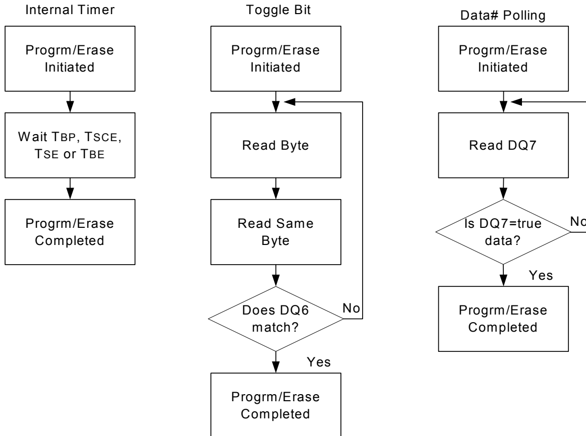
Figure 13: Wait Options
