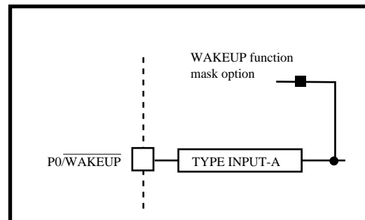
TYPE INPUT-B
