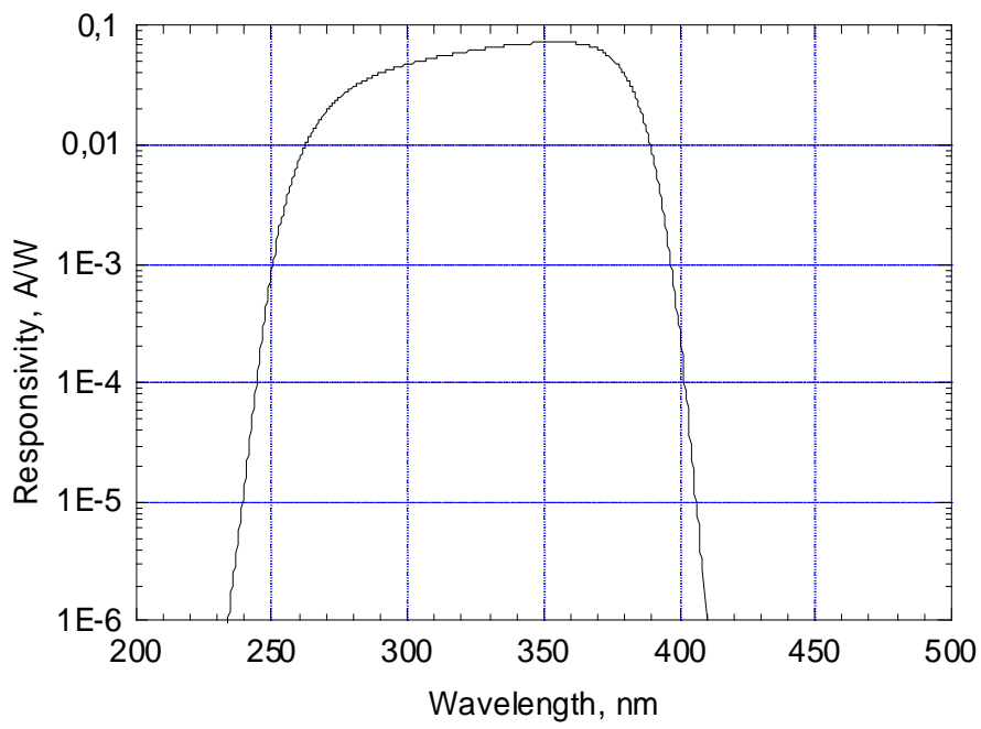
Typical responsivity
