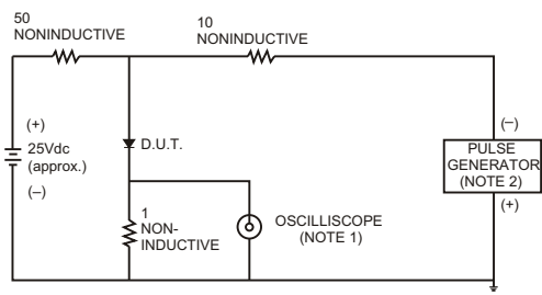
FIG.1- TEST CIRCUIT DIAGRAM AND REVERSE RECOVERY CHARACTERISTIC
