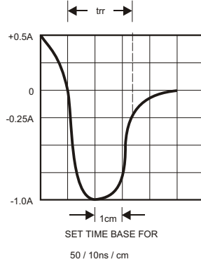
FIG.1- TEST CIRCUIT DIAGRAM AND REVERSE RECOVERY CHARACTERISTIC
