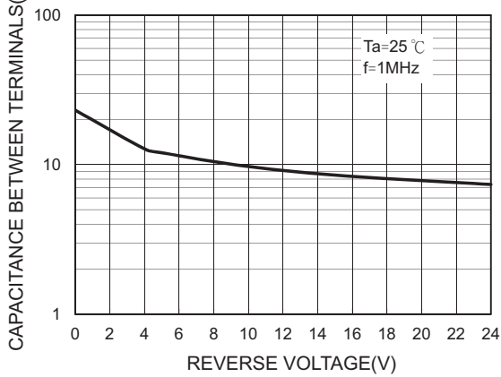
FIG.3- TERMINALS CHARACTERISTICS
