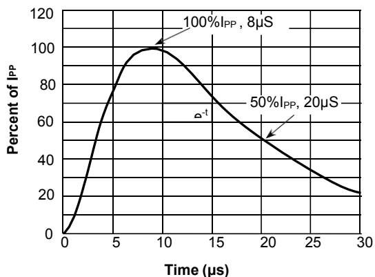
Fig.3 Pulse Waveform-8/20μs
