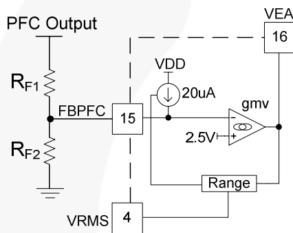
Figure 46. Two-Level PFC Scheme
