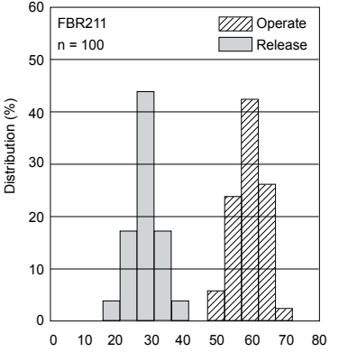
Nominal voltage multiplying factor (%)
