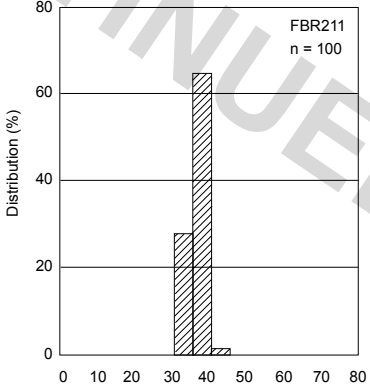
Contact resistance (mΩ)
