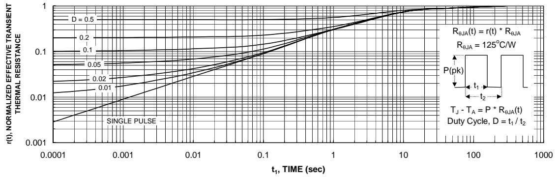
Figure 11. Transient Thermal Response Curve. Thermal characterization performed using the conditions described in Note 1c. Transient thermal response will change depending on the circuit board design.
