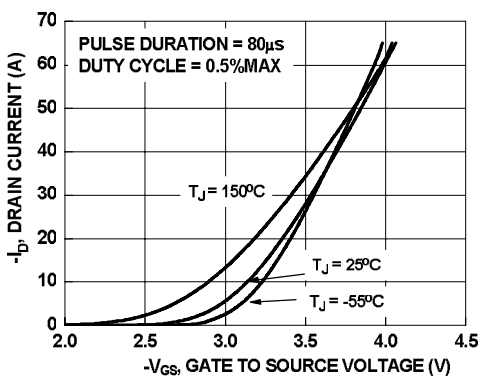
Figure 5. Transfer Characteristics
