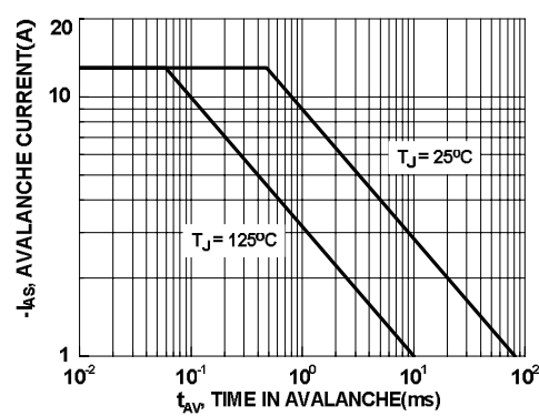
Figure 10. Unclamped Inductive Switching Capability
