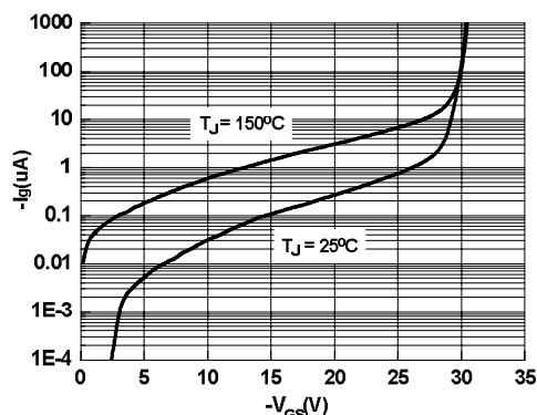
Figure 9. I_g vs V_{GS}
