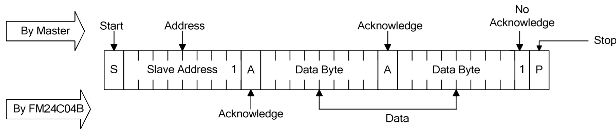
Figure 8. Sequential Read
