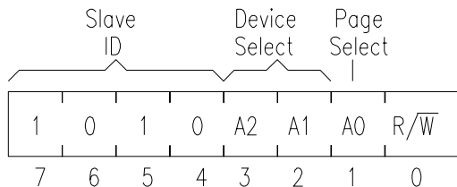
Figure 4. Slave Address
