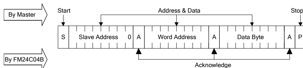
Figure 5. Byte Write
