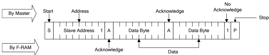
Figure 8. Sequential Read
