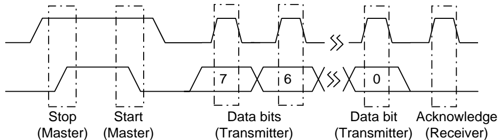
Figure 3. Data Transfer Protocol
