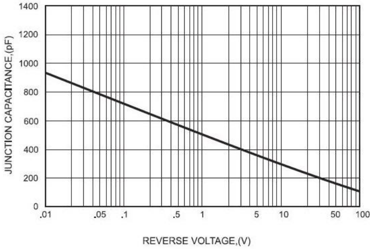
FIG.4-TYPICAL JUNCTION CAPACITANCE
