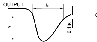
Fig.8 Reverse recovery time (t rr ) measurement circuit
