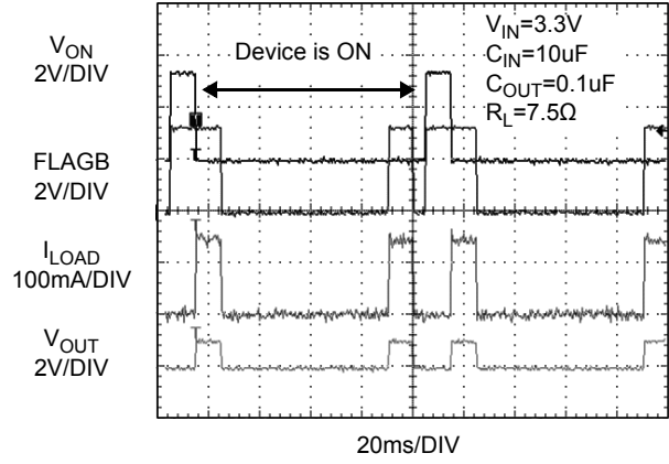
Figure 20. PPF2025 T_{BLANK} and T_{RESTART} (Active LO Device)
