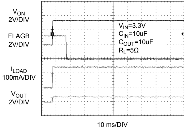
Figure 19. PPF2027 Startup FLAGB Blanking Time
