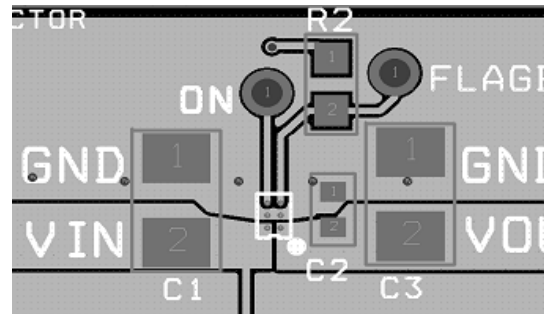
Figure 24. FPF202X proper layout
