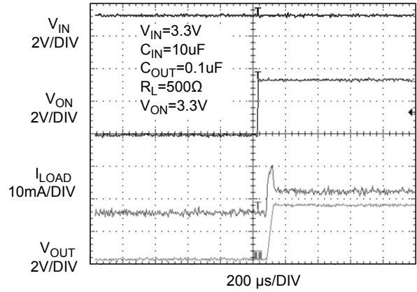
Figure 10. FPF2024 T_{ON} Response
