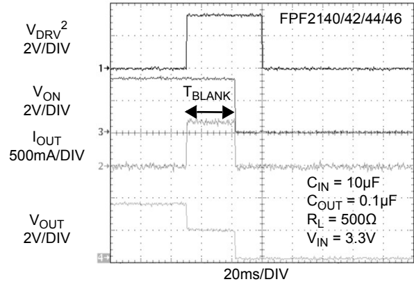
Figure 22. T_{BLANK} Response
