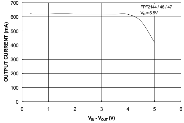
Figure 8. Current
