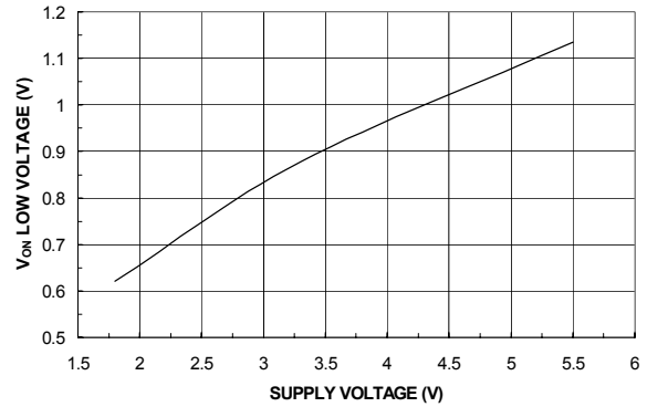
Figure 4. V ON Low Voltage vs. Input Voltage
