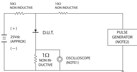
FIG.5-TEST CIRCUIT DIAGRAM AND REVERSE RECOVERY TIME CHARACTERISTIC
