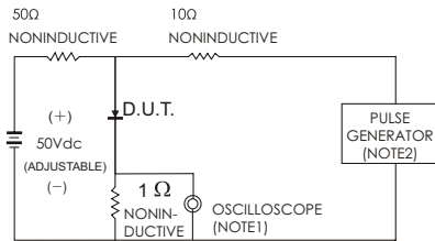
FIG.5-TEST CIRCUIT DIAGRAM AND REVERSE RECOVERY TIME CHARACTERISTIC
