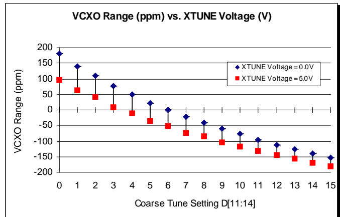
Figure 3: VCXO Range
