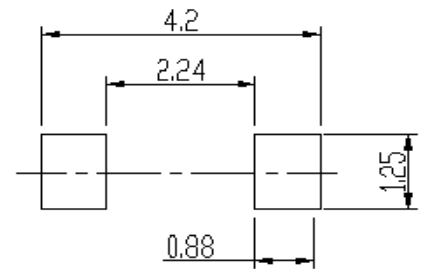
Soldering footprint
