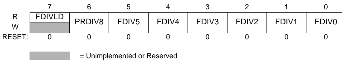
Figure 3-2 Flash Clock Divider Register (FCLKDIV)
