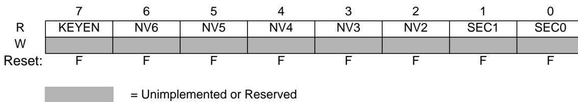
Figure 3-3 Flash Security Register (FSEC)
