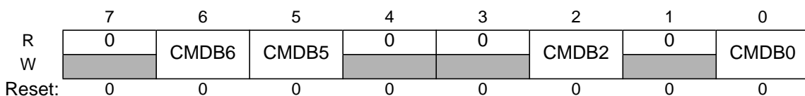
Figure 3-8 Flash Command Buffer and Register (FCMD)
