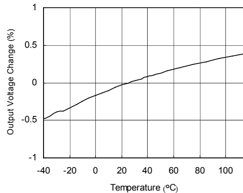
Temperature Stability
