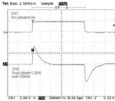
Line transient
