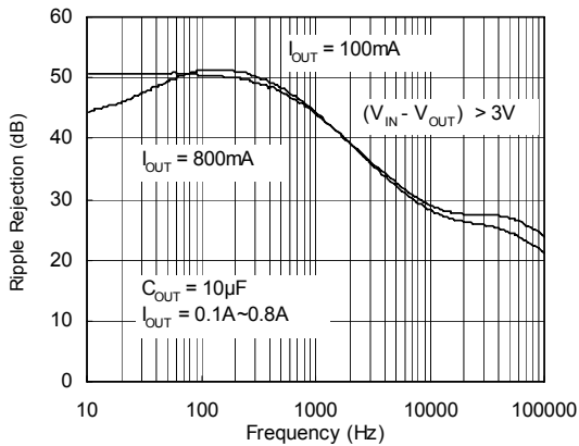
Ripple Rejection
