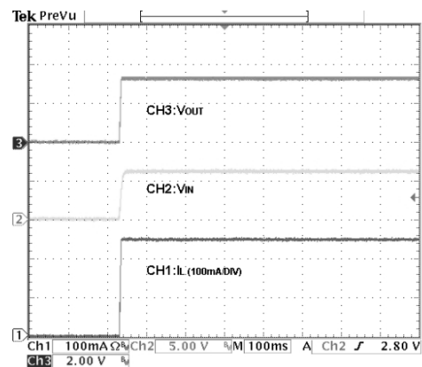
Start-UP (SOT-89)
