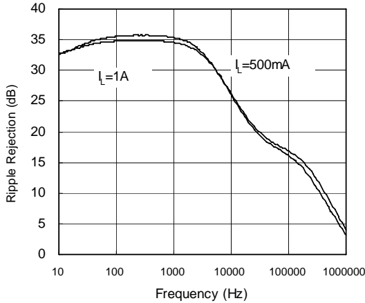
Ripple Rejection
