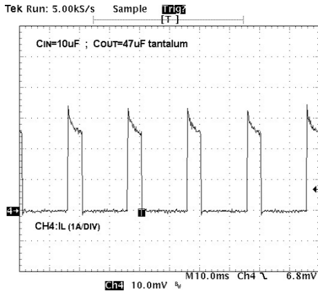
Short Circuit-Current
