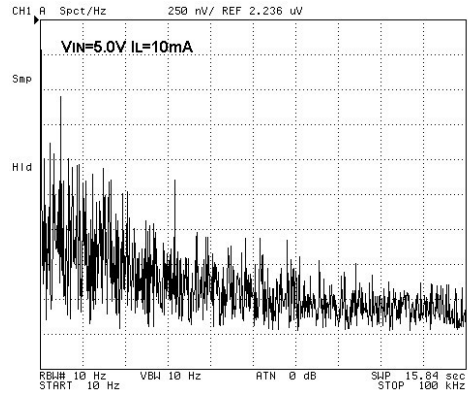
Output Noise
