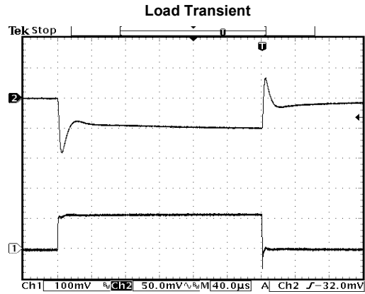
Ch1: Iout (400mA/div) Ch2: Vout (offset=3.50V)
