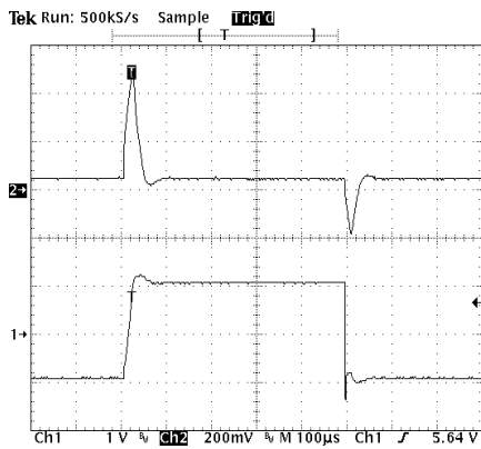
Line Transient
