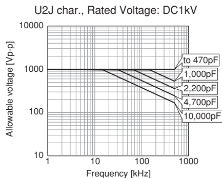
Sine-wave frequency VS allowable voltage
